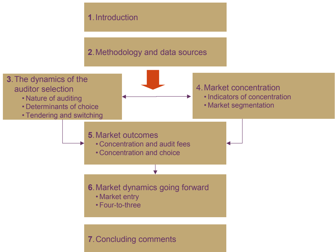
Figure 1.3 Report structure
